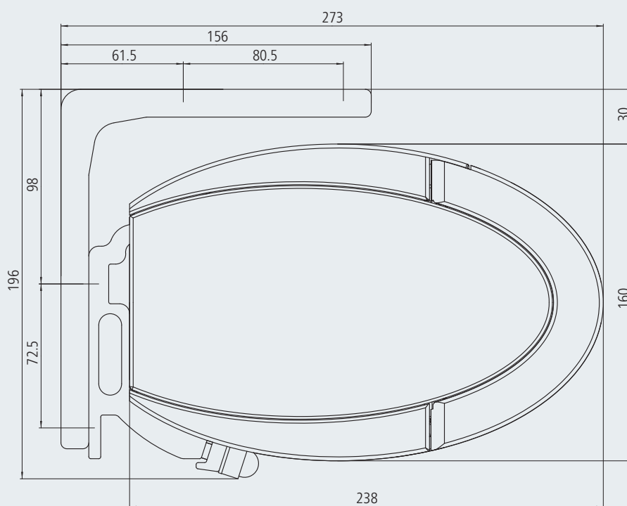
Side view with ceiling bracket
