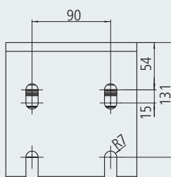
Ceiling bracket
