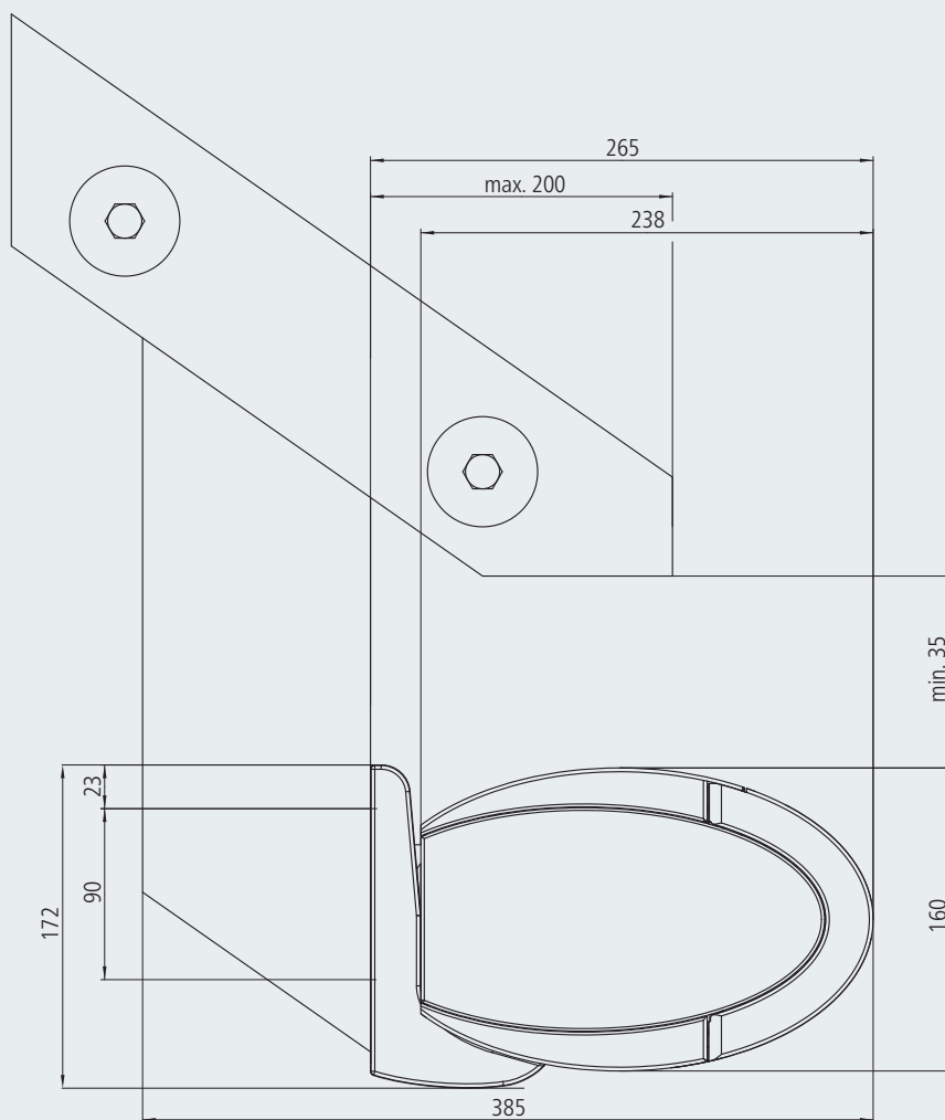
Side view: mounting rafter bracket
